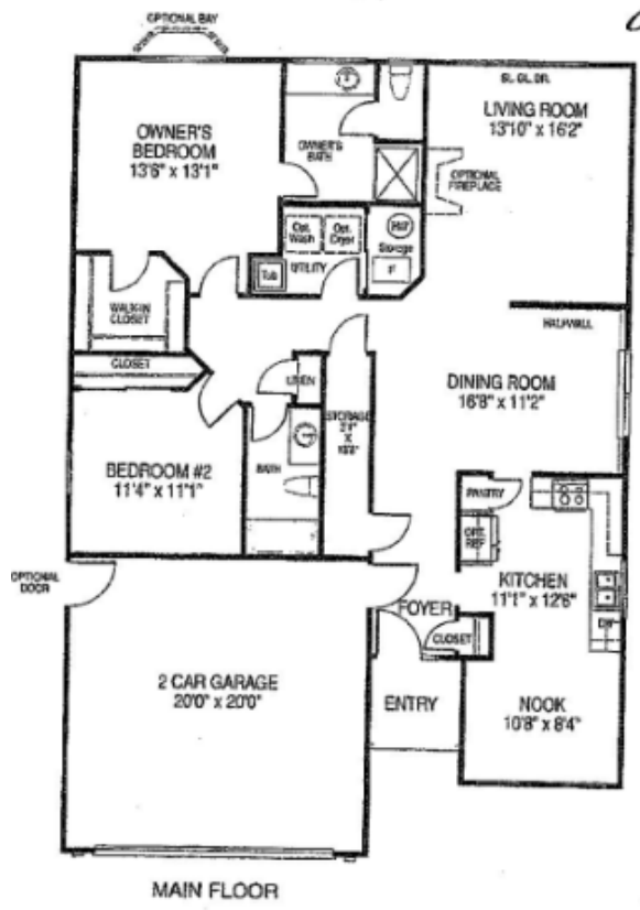
1ST FLOOR PLAN WITH BASEMENT
